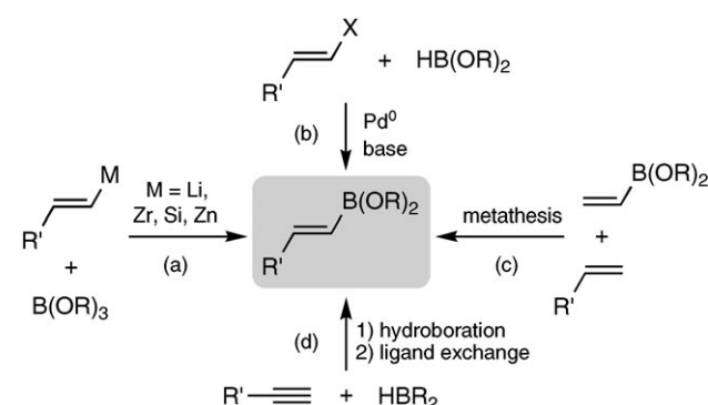
Scheme 1. Routes to alkenyl boronates: a) Quenching of alkenyl metal species. b) Pd-catalyzed halogen/boron exchange. c) Olefin metathesis. d) Hydroboration.
